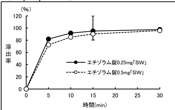
<50rpm: pH6.8>
