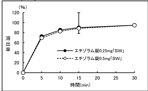
<50rpm: pH4.0>
